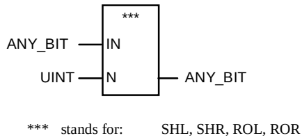
Figure A.5. Graphical declarations of the bit-shift functions SHL, SHR, ROR and ROL
