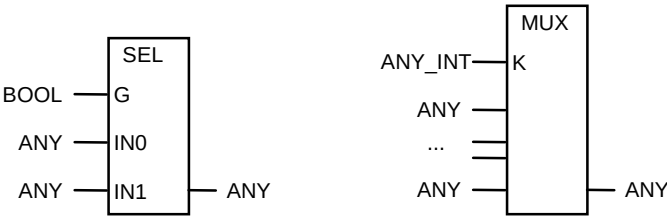
Figure A.8. Graphical declarations of the selection functions SEL and MUX
