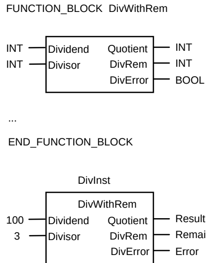
Example C.6. Graphical declaration part for Example C.4 (top) and example of a call of the FB instance DivInst (bottom)
