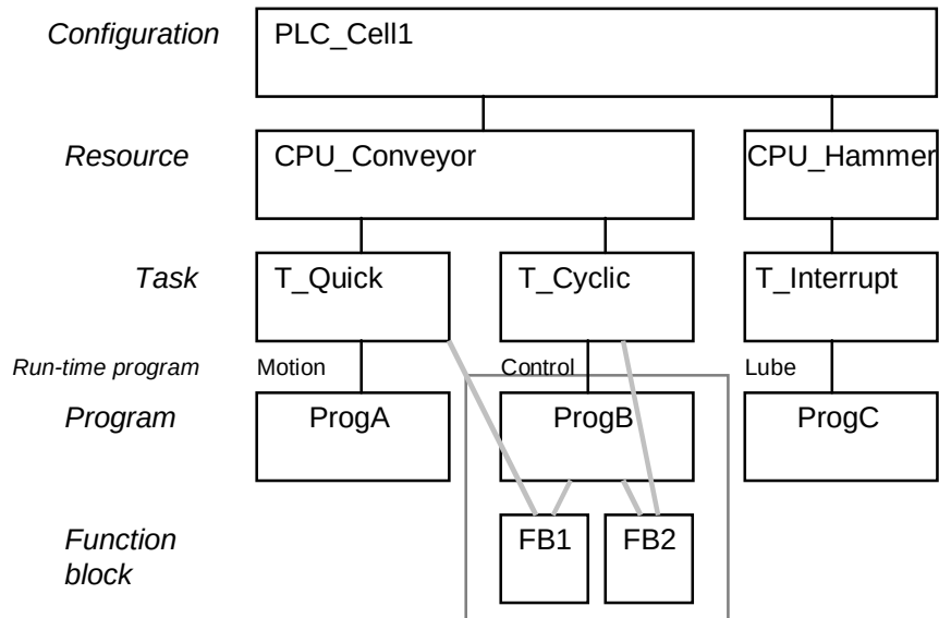
Example 6.5. Example of configuration elements with POU (overview)
